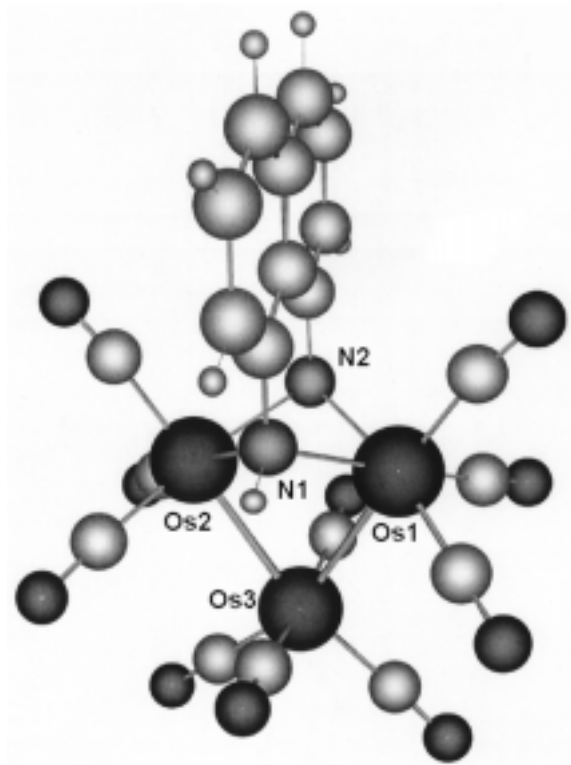
Figure 3. Molecular structure of compound 3
